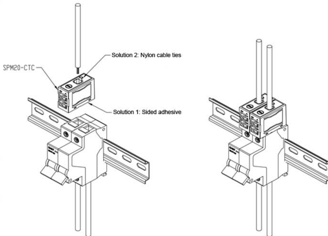
Figure 4: Controller installation
