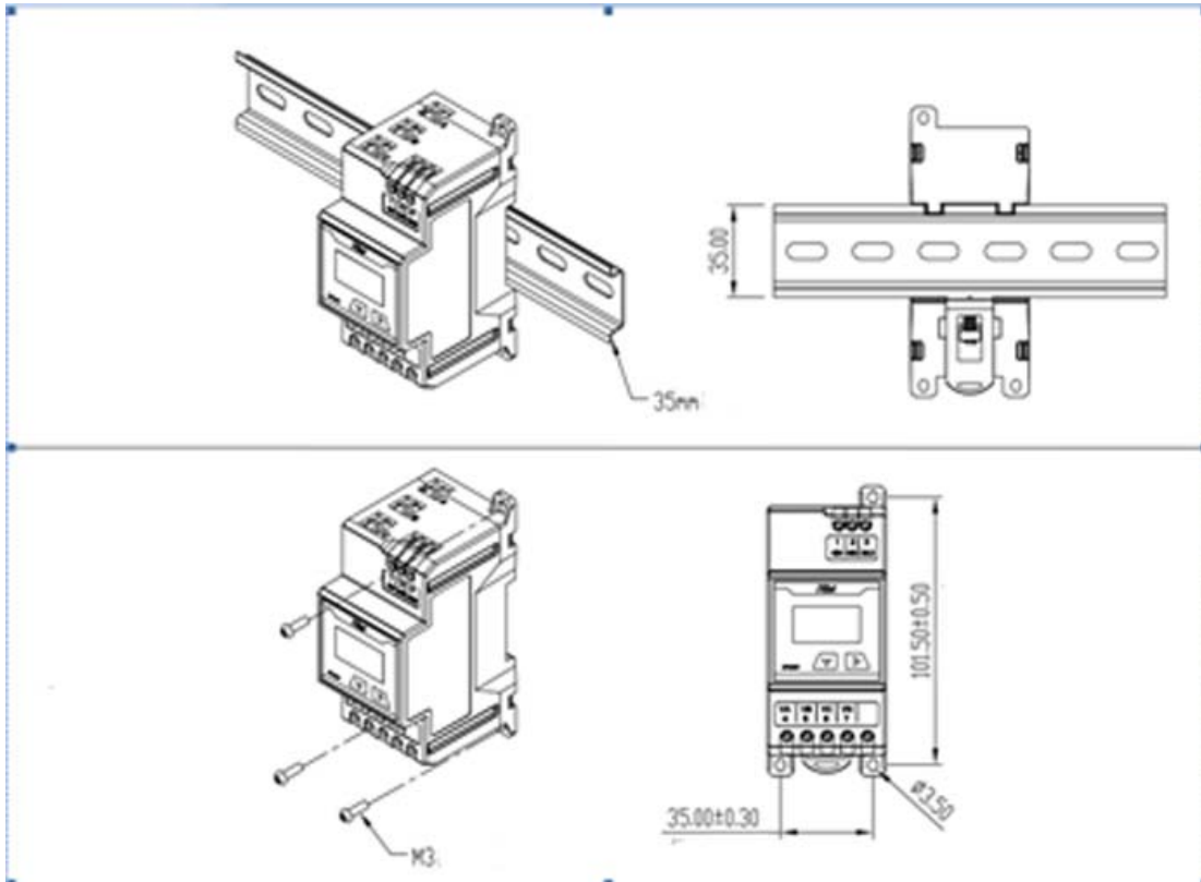
Figure 4: Controller installation
