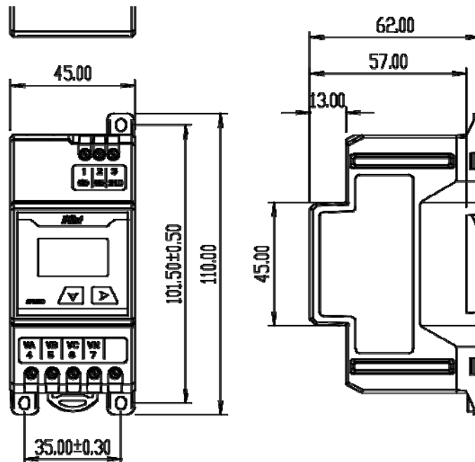
Figure 1 : controller dimension
