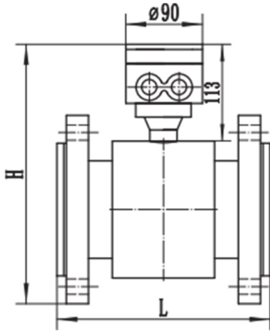
1/2"-24" Remote Electromagnetic Flow Meter with ANSI 150# Drawing
