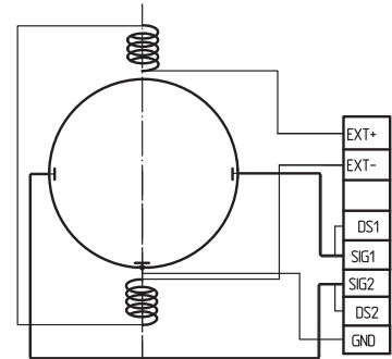
Electromagnetic Flowmeter Circuit
