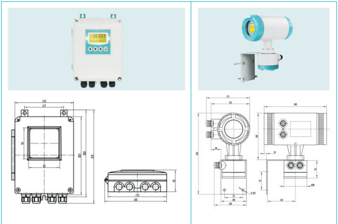
Remote Transmitter
